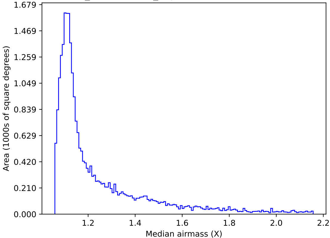
weather_cloudso2v3.4_10yrs Yr 1 r band: Median airmass
