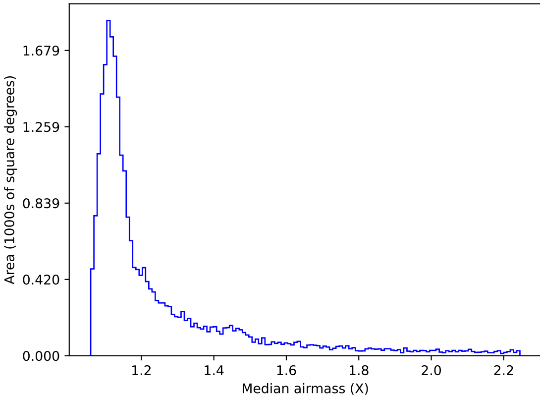
weather_cloudso2v3.4_10yrs Yr 1 i band: Median airmass
