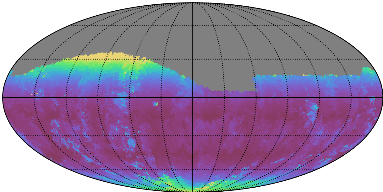
weather_cloudso2v3.4_10yrs Yr 1 g band: Median airmass
