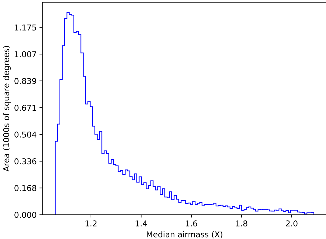
weather_cloudso2v3.4_10yrs Yr 1 g band: Median airmass
