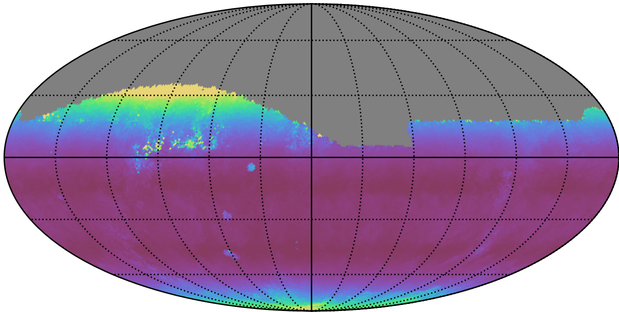
weather_cloudso2v3.4_10yrs Yr 1 all bands: Median airmass
