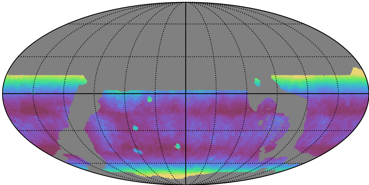
weather_cloudso2v3.4_10yrs WFD z band: Median airmass
