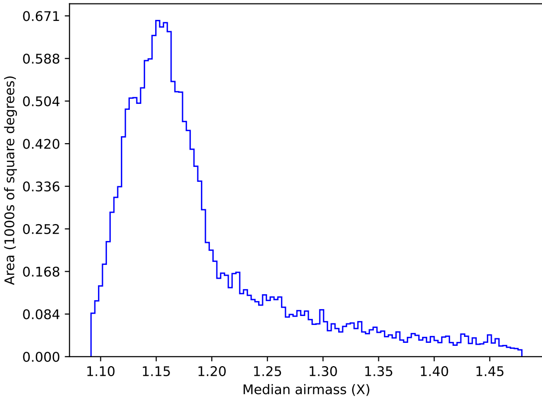
weather_cloudso2v3.4_10yrs WFD z band: Median airmass
