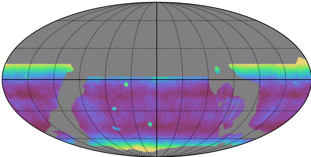
weather_cloudso2v3.4_10yrs WFD y band: Median airmass
