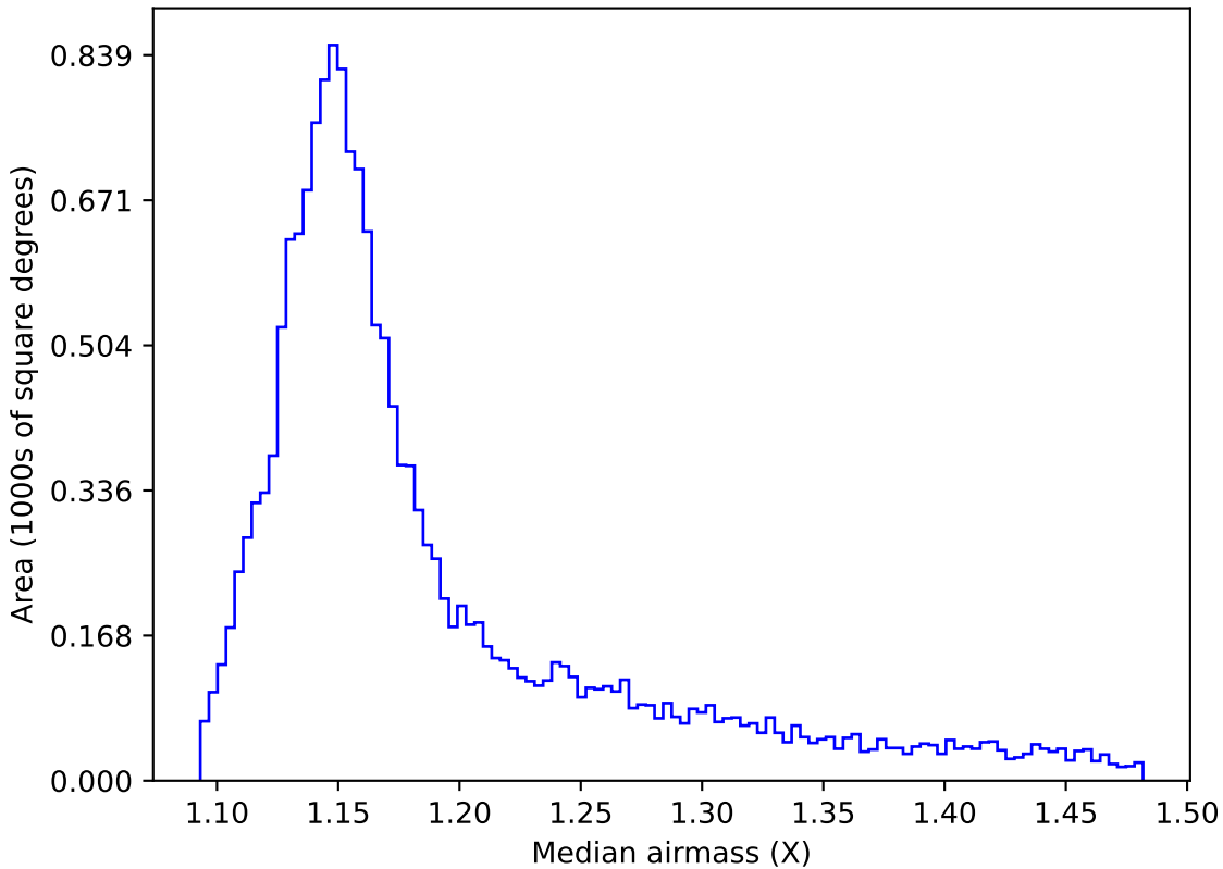
weather_cloudso2v3.4_10yrs WFD y band: Median airmass
