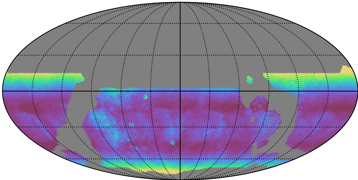
weather_cloudso2v3.4_10yrs WFD u band: Median airmass
