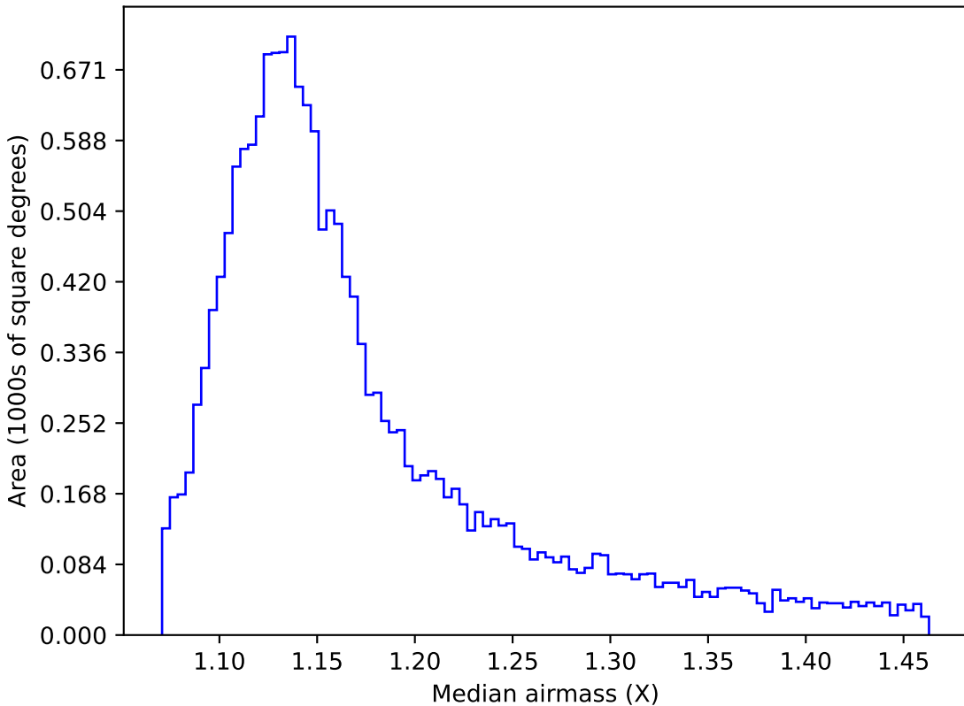
weather_cloudso2v3.4_10yrs WFD u band: Median airmass
