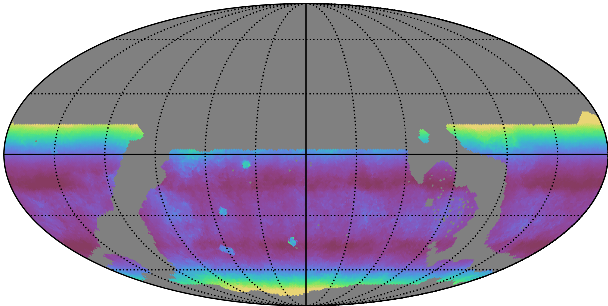
weather_cloudso2v3.4_10yrs WFD r band: Median airmass
