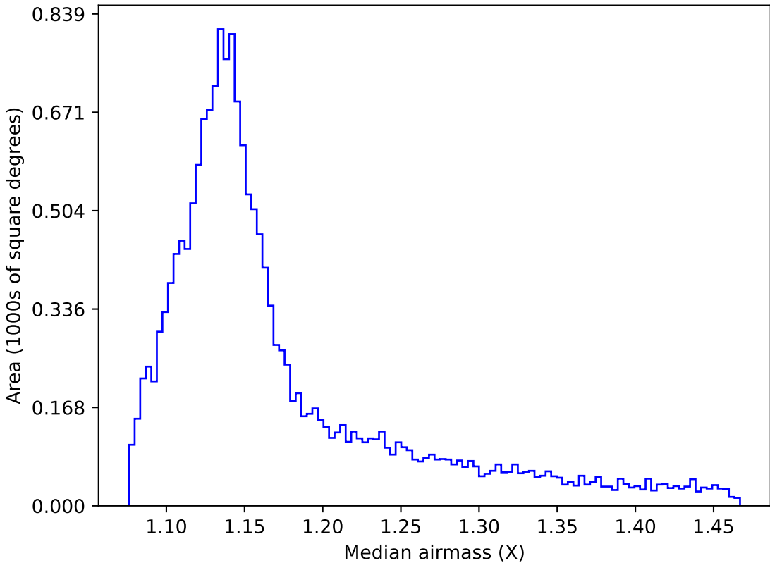
weather_cloudso2v3.4_10yrs WFD r band: Median airmass
