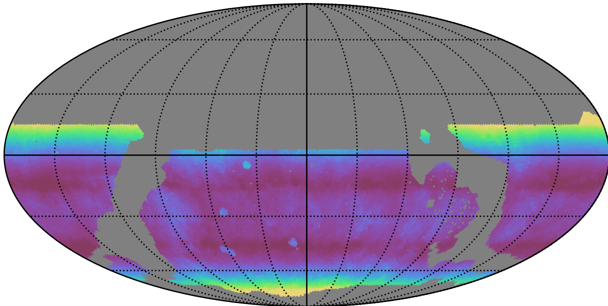
weather_cloudso2v3.4_10yrs WFD i band: Median airmass
