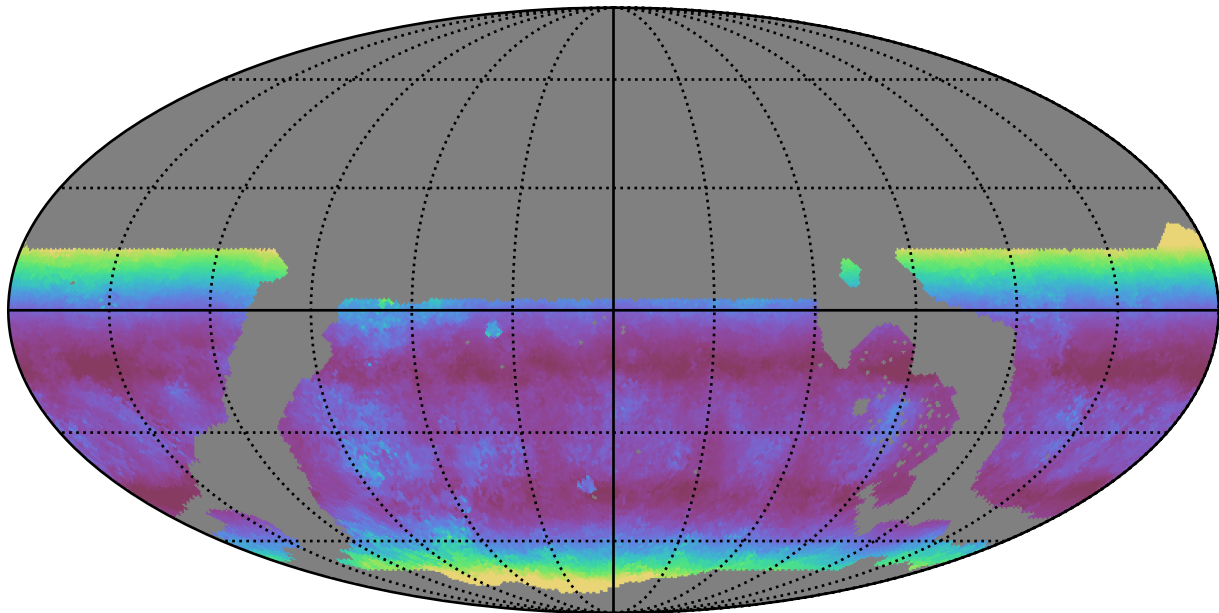
weather_cloudso2v3.4_10yrs WFD g band: Median airmass
