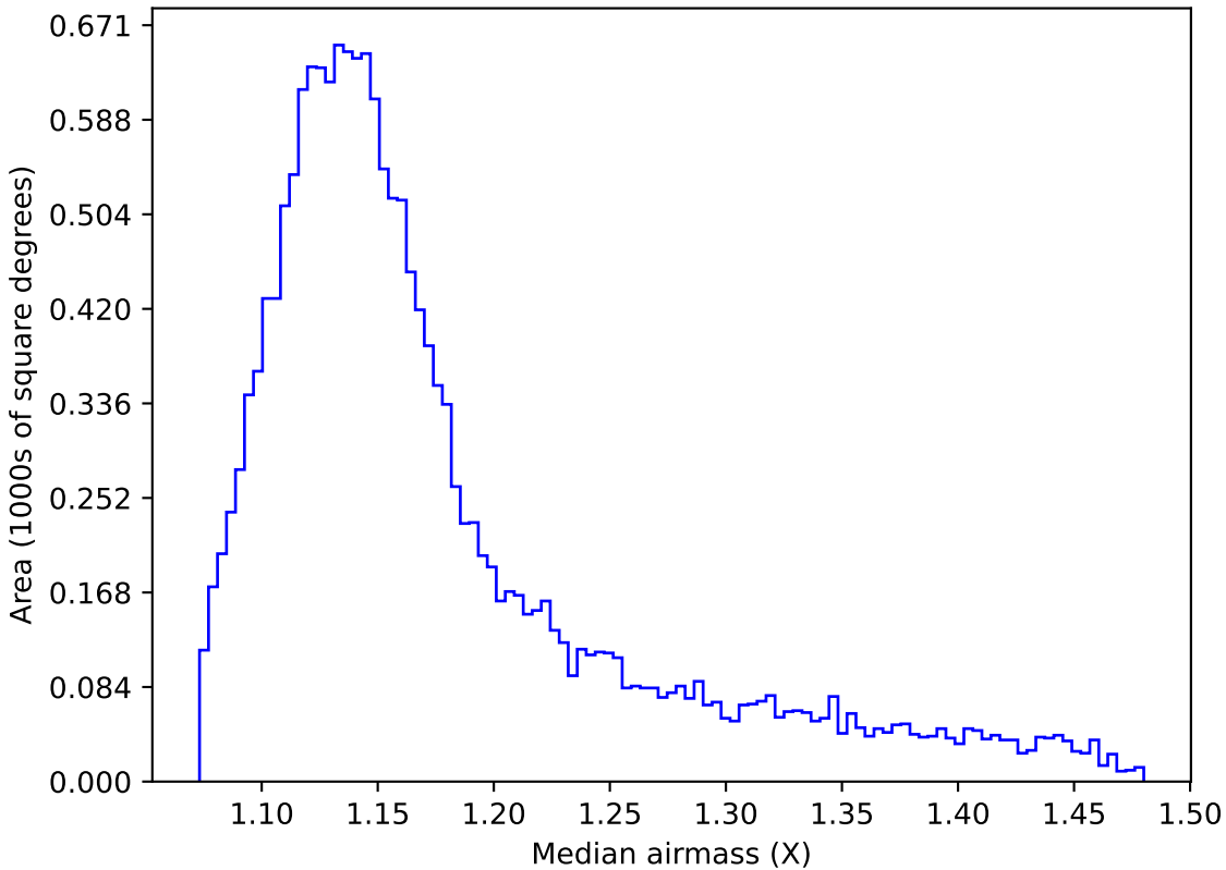
weather_cloudso2v3.4_10yrs WFD g band: Median airmass
