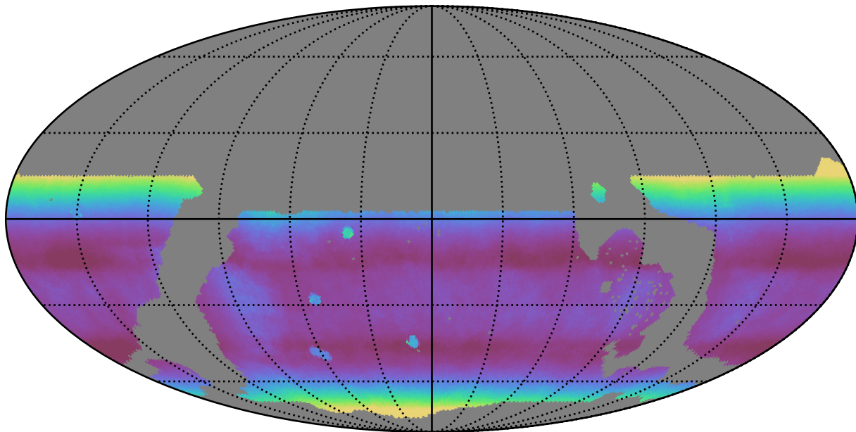
weather_cloudso2v3.4_10yrs WFD all bands: Median airmass
