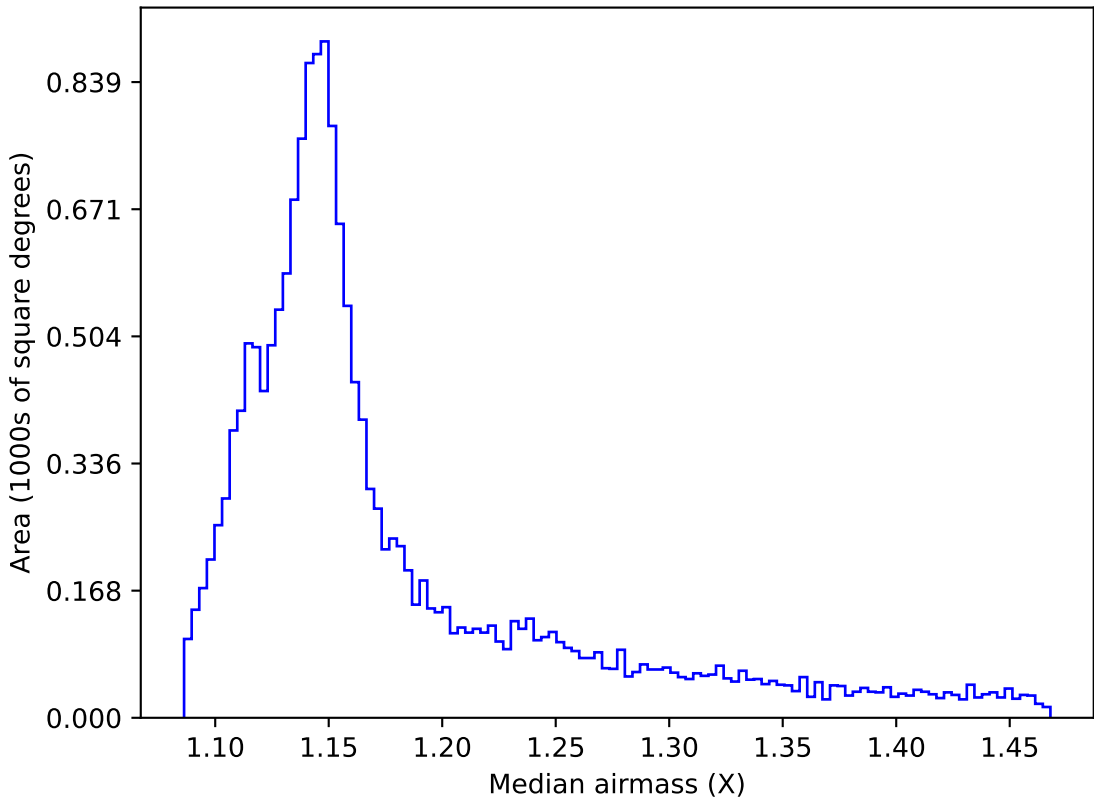
weather_cloudso2v3.4_10yrs WFD all bands: Median airmass
