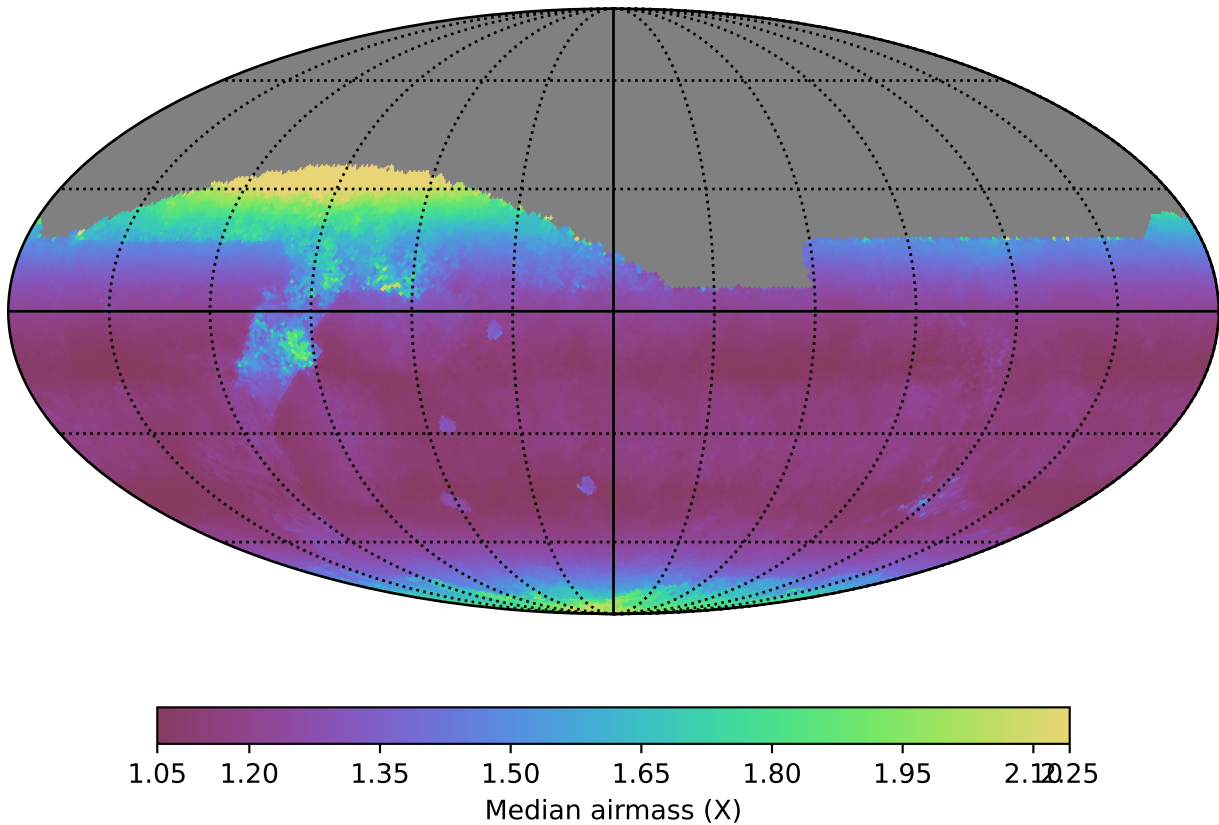
weather_cloudso2v3.4_10yrs All sky z band: Median airmass
