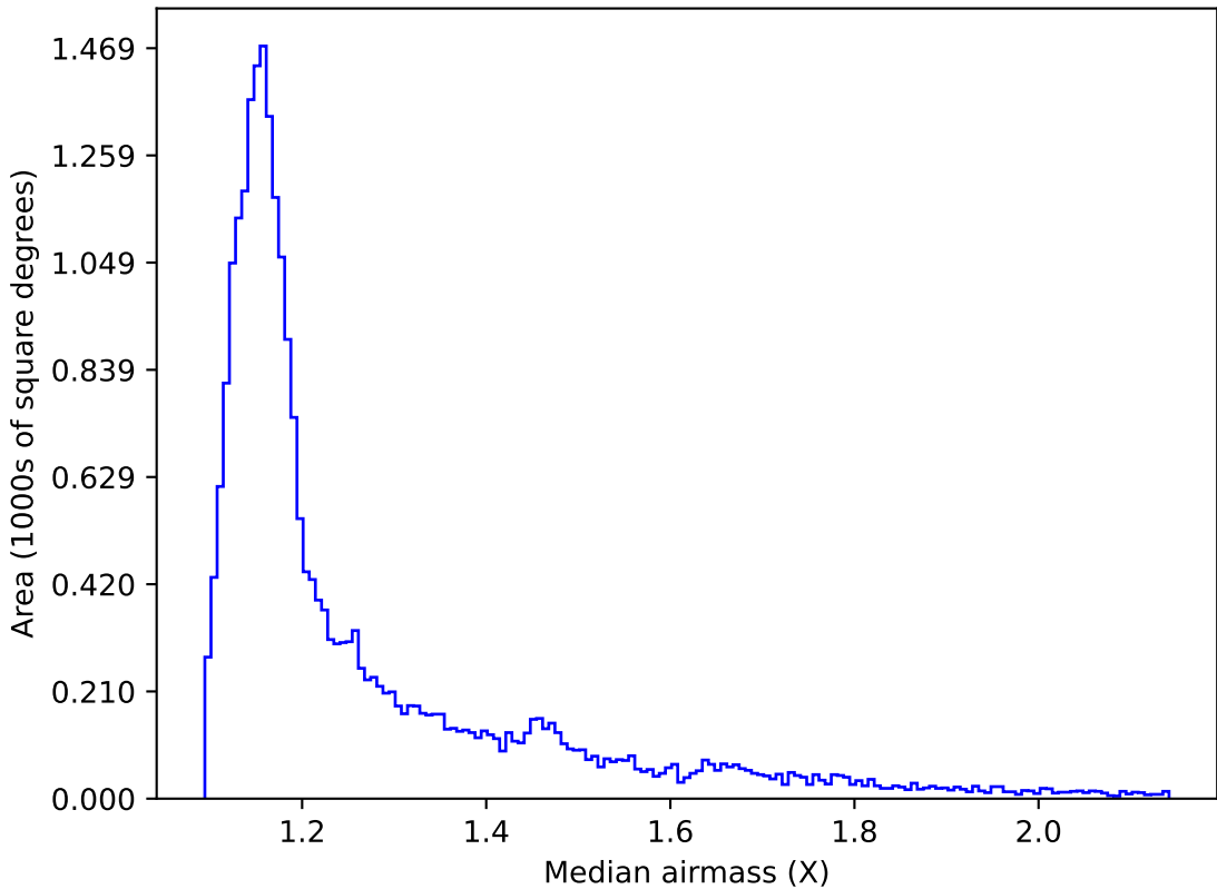
weather_cloudso2v3.4_10yrs All sky z band: Median airmass
