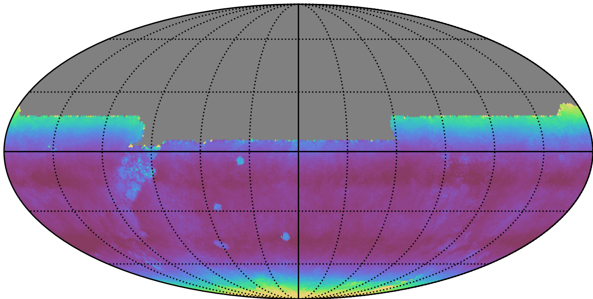
weather_cloudso2v3.4_10yrs All sky y band: Median airmass
