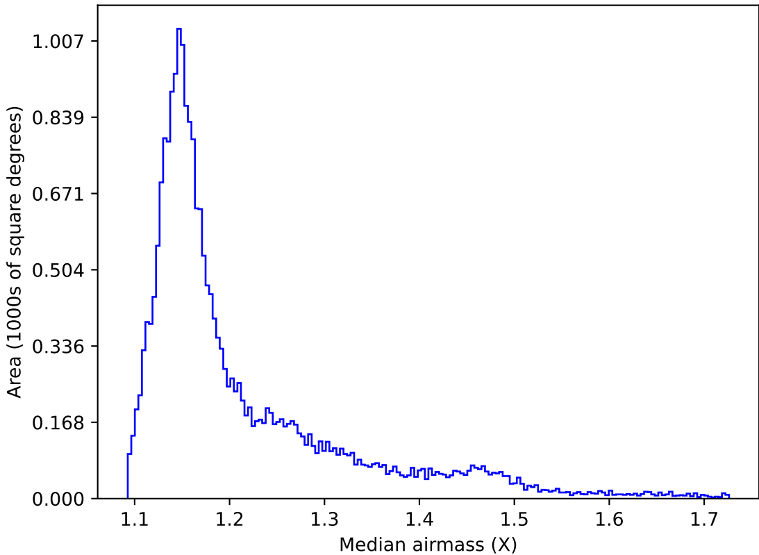
weather_cloudso2v3.4_10yrs All sky y band: Median airmass
