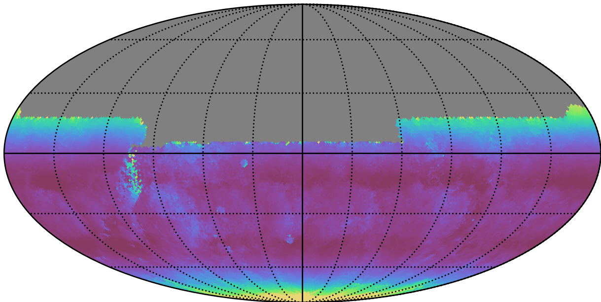
weather_cloudso2v3.4_10yrs All sky u band: Median airmass
