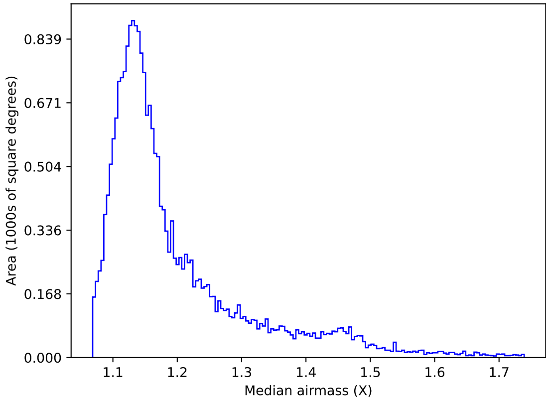
weather_cloudso2v3.4_10yrs All sky u band: Median airmass
