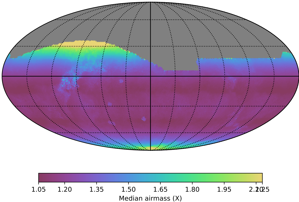
weather_cloudso2v3.4_10yrs All sky r band: Median airmass
