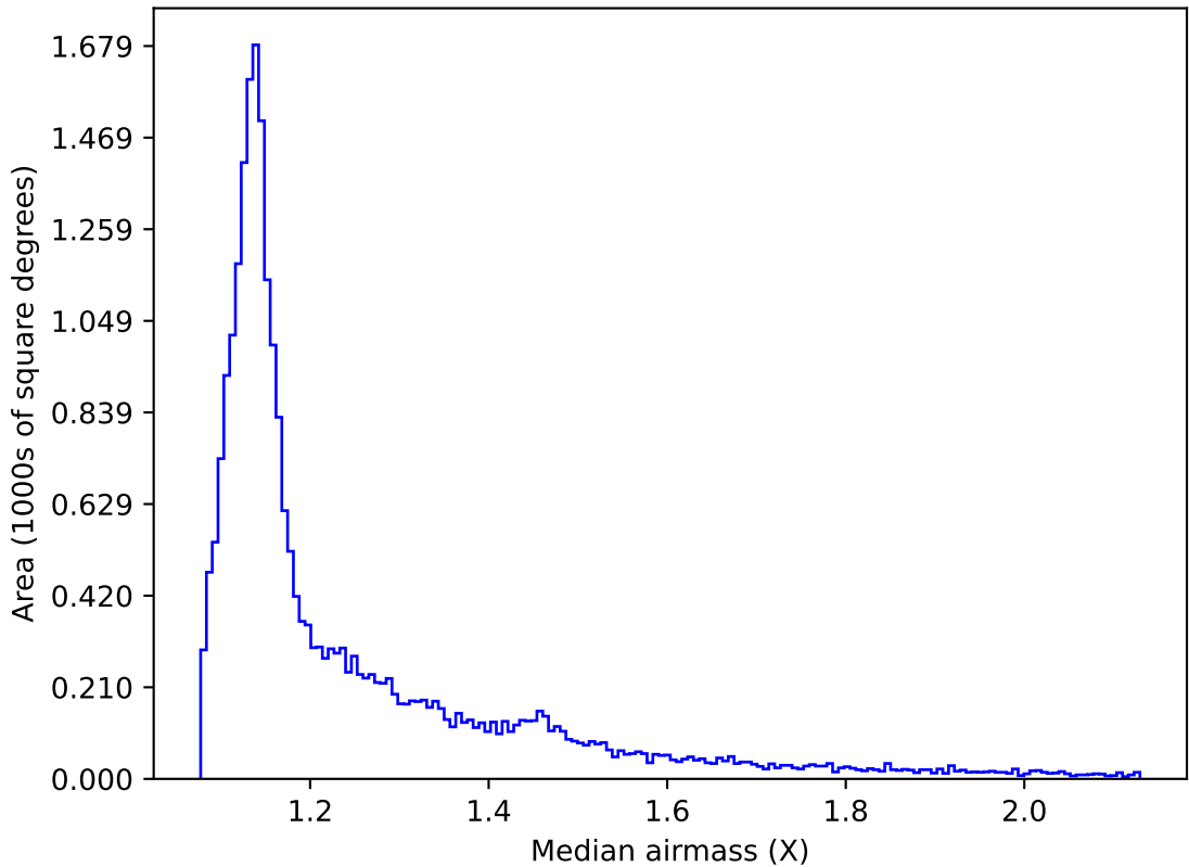
weather_cloudso2v3.4_10yrs All sky r band: Median airmass
