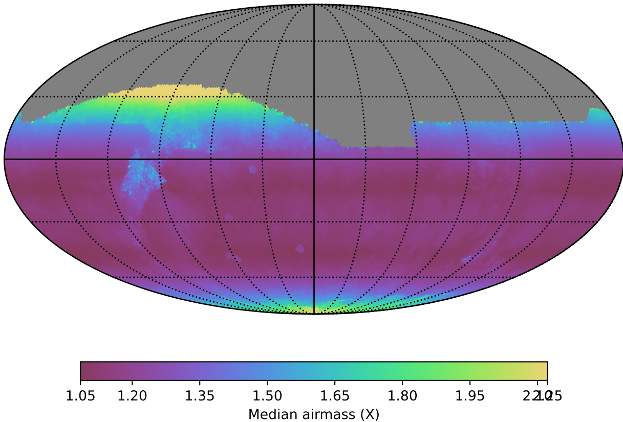
weather_cloudso2v3.4_10yrs All sky i band: Median airmass
