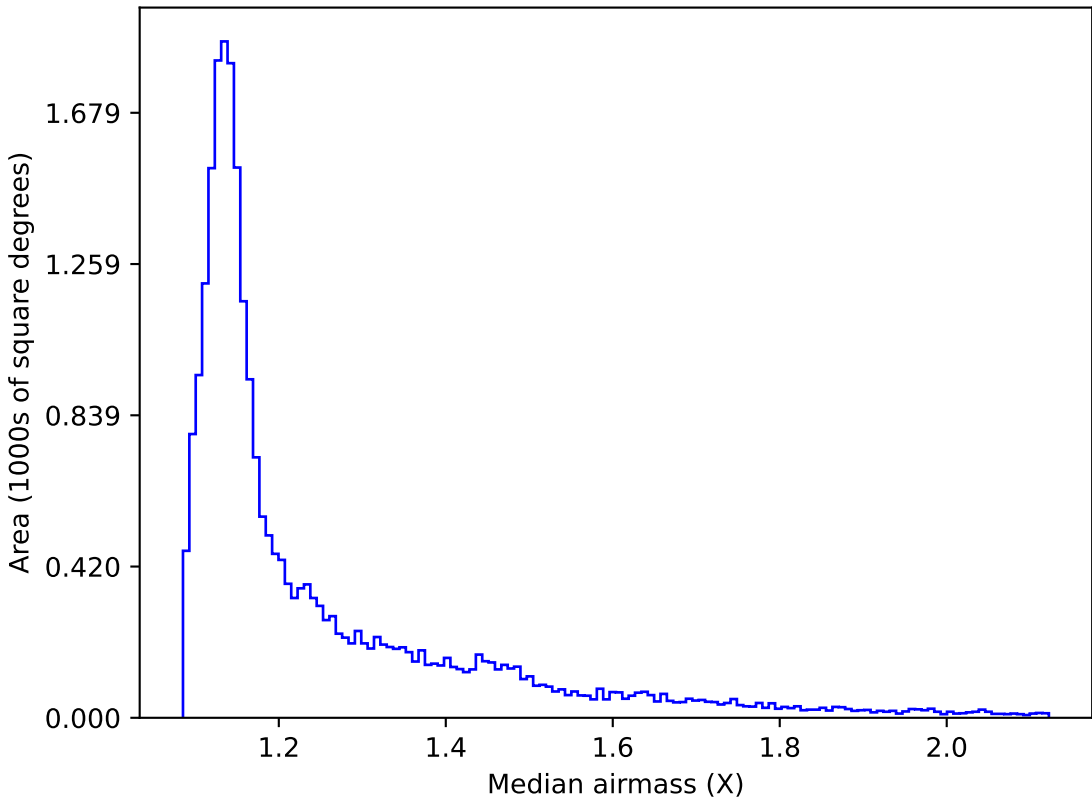
weather_cloudso2v3.4_10yrs All sky i band: Median airmass
