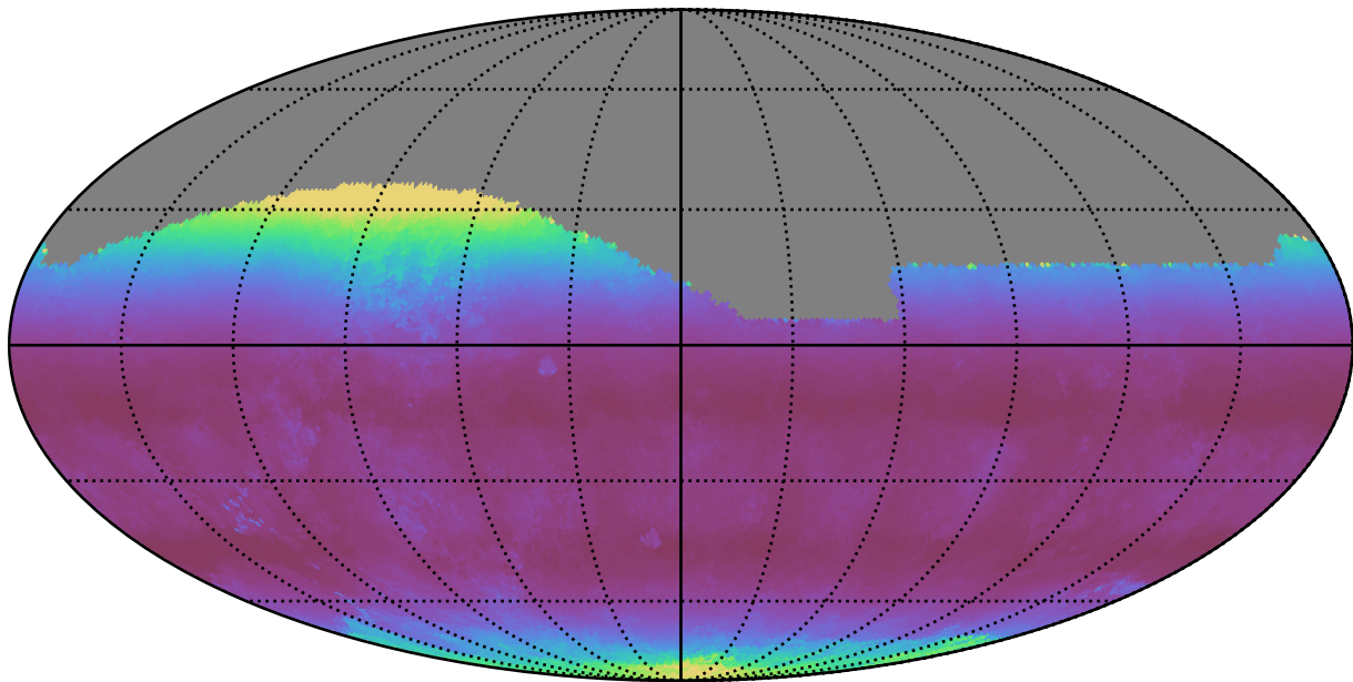
weather_cloudso2v3.4_10yrs All sky g band: Median airmass
