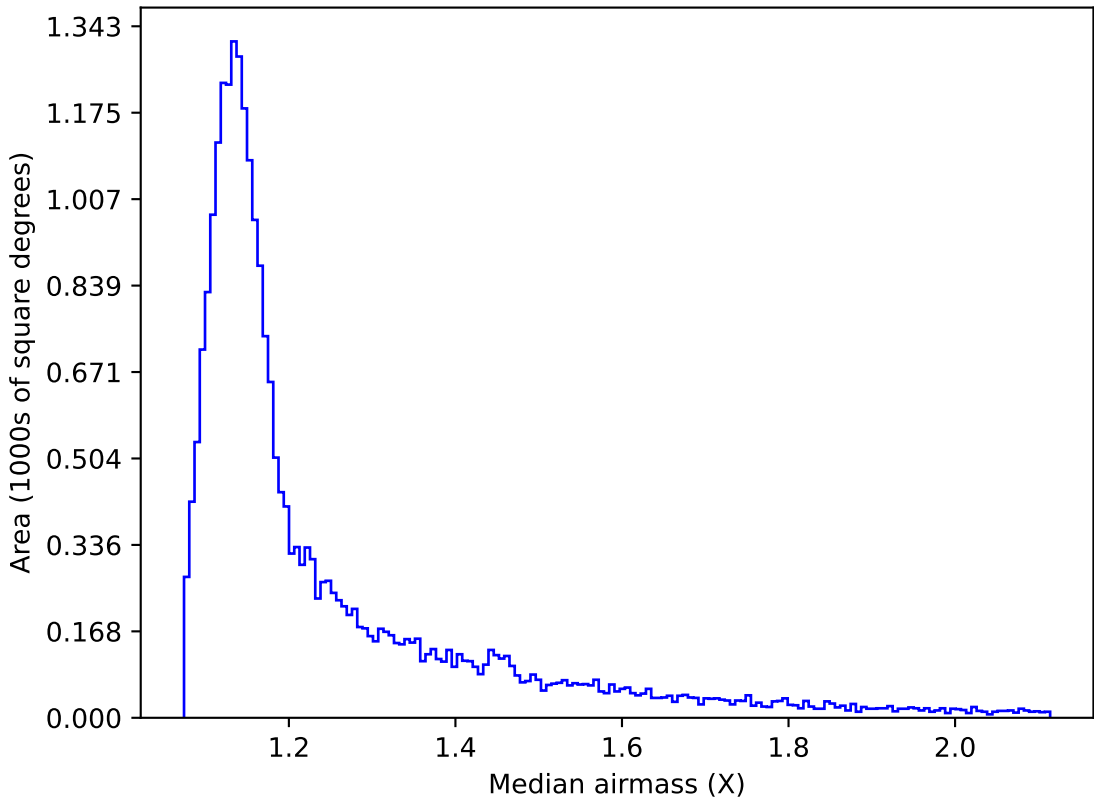
weather_cloudso2v3.4_10yrs All sky g band: Median airmass
