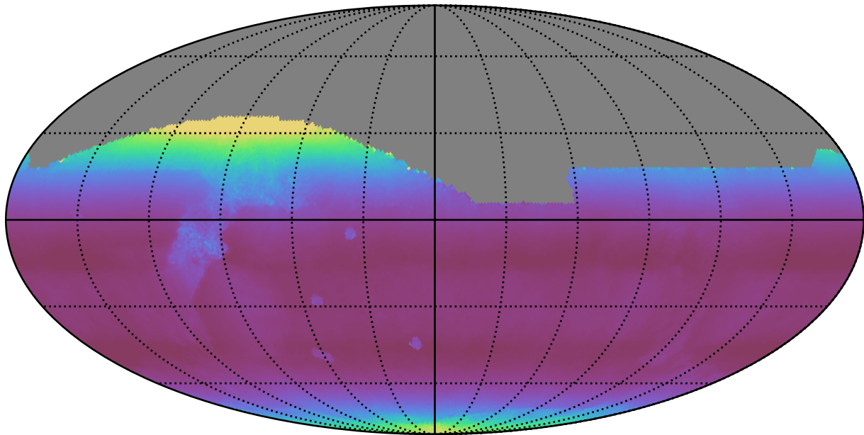
weather_cloudso2v3.4_10yrs All sky all bands: Median airmass
