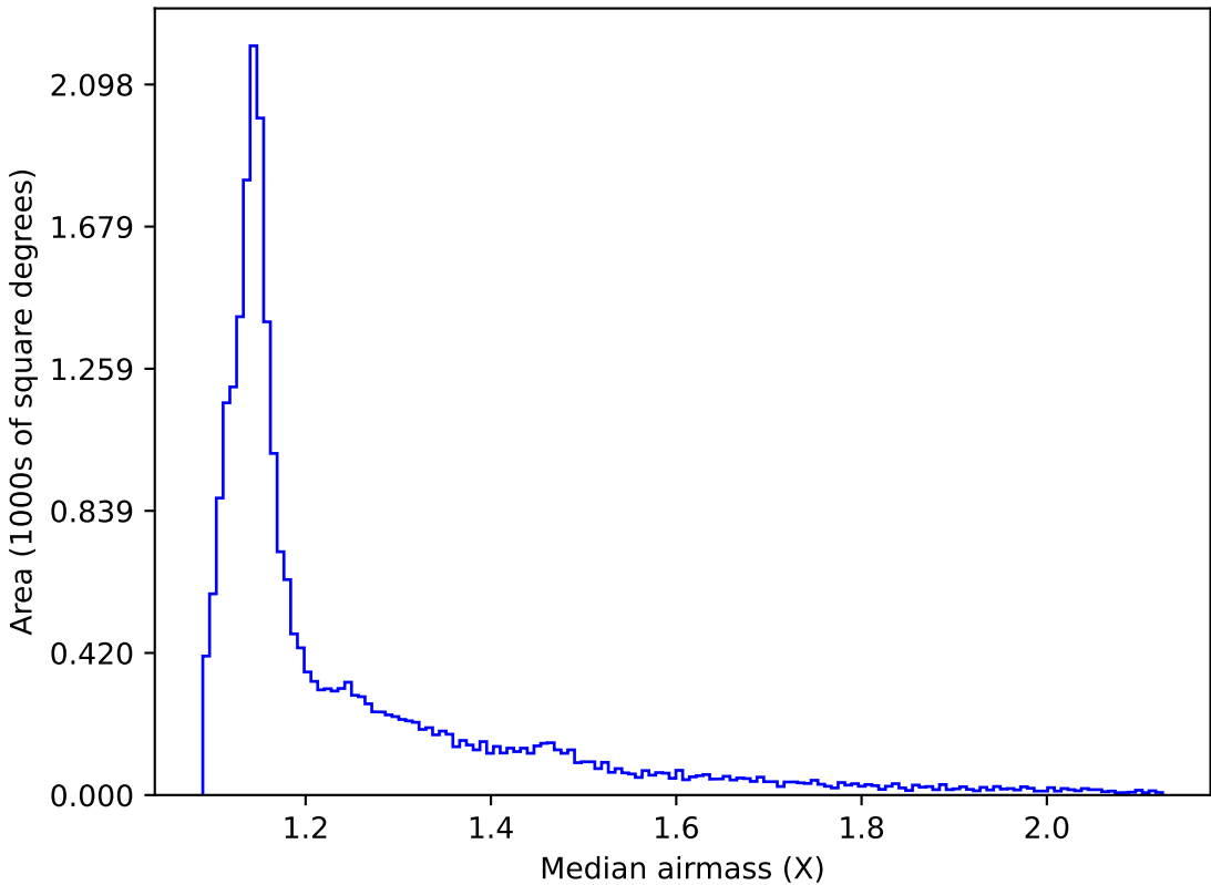
weather_cloudso2v3.4_10yrs All sky all bands: Median airmass
