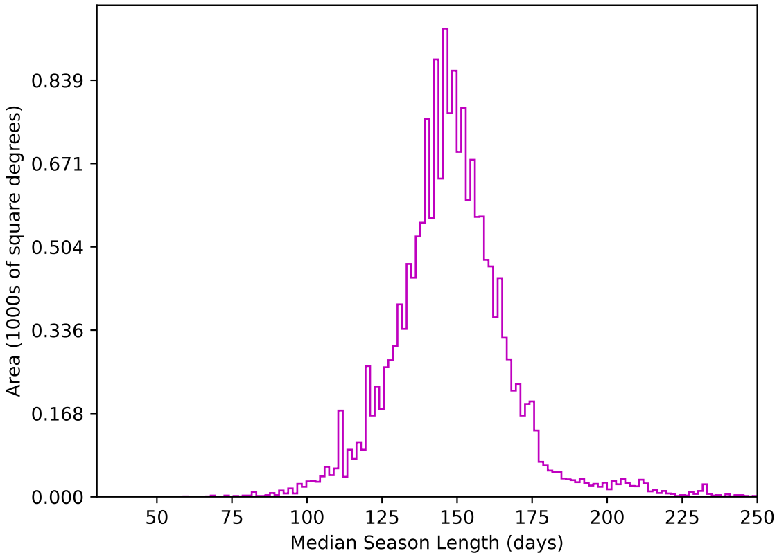
weather_cloudso2v3.4_10yrs WFD z band: Median Season Length
