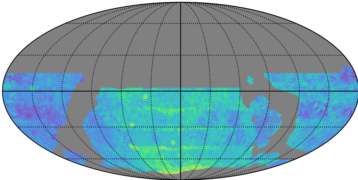
weather_cloudso2v3.4_10yrs WFD y band: Median Season Length
