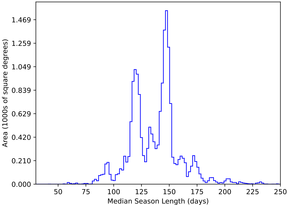
weather_cloudso2v3.4_10yrs WFD y band: Median Season Length
