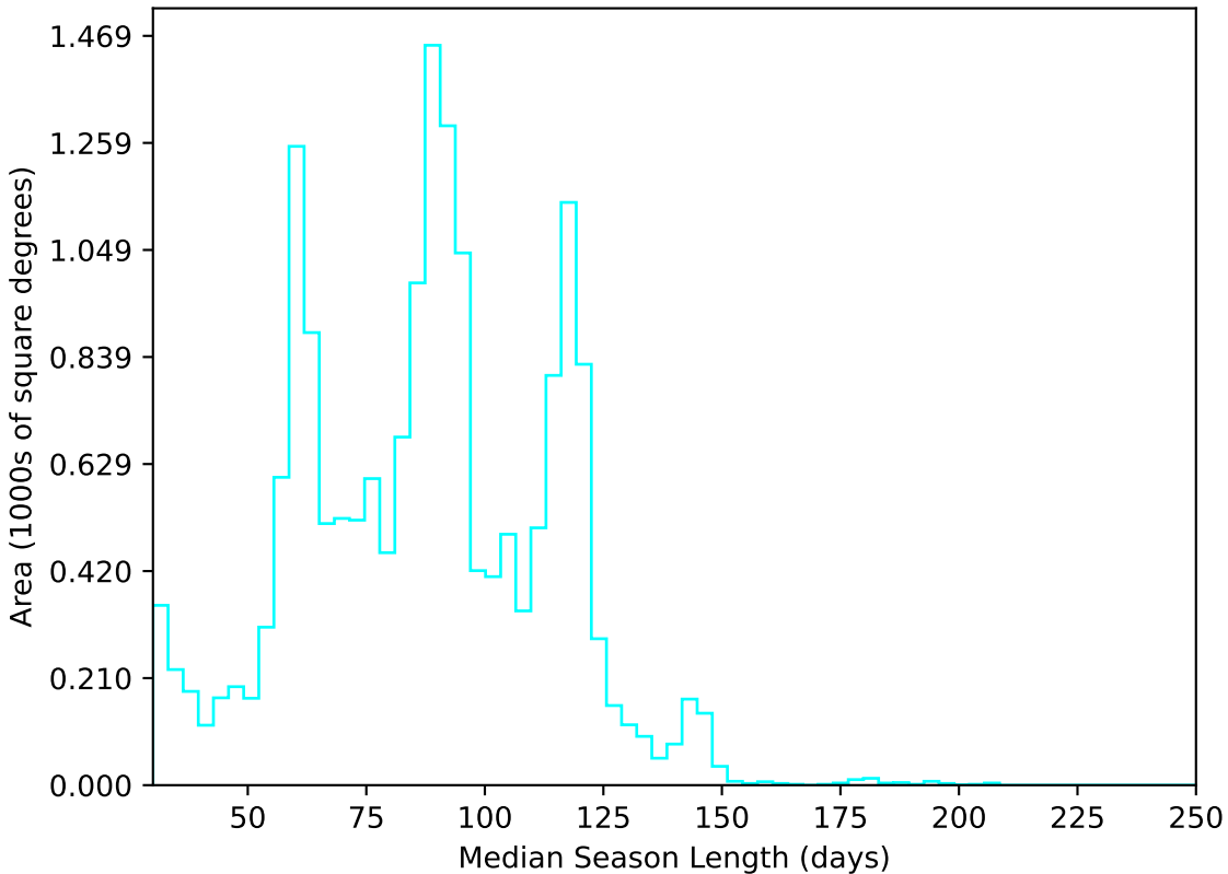
weather_cloudso2v3.4_10yrs WFD u band: Median Season Length
