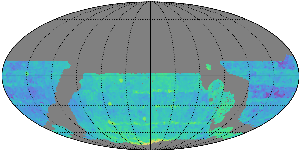
weather_cloudso2v3.4_10yrs WFD i band: Median Season Length
