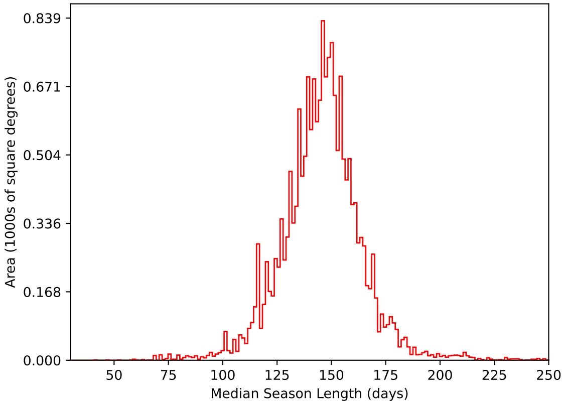
weather_cloudso2v3.4_10yrs WFD i band: Median Season Length
