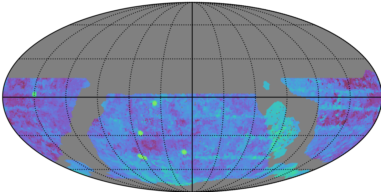
weather_cloudso2v3.4_10yrs WFD g band: Median Season Length
