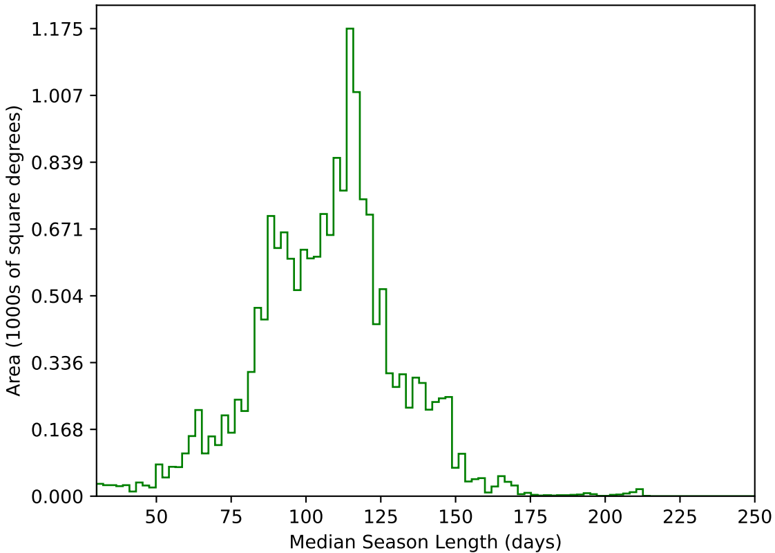
weather_cloudso2v3.4_10yrs WFD g band: Median Season Length
