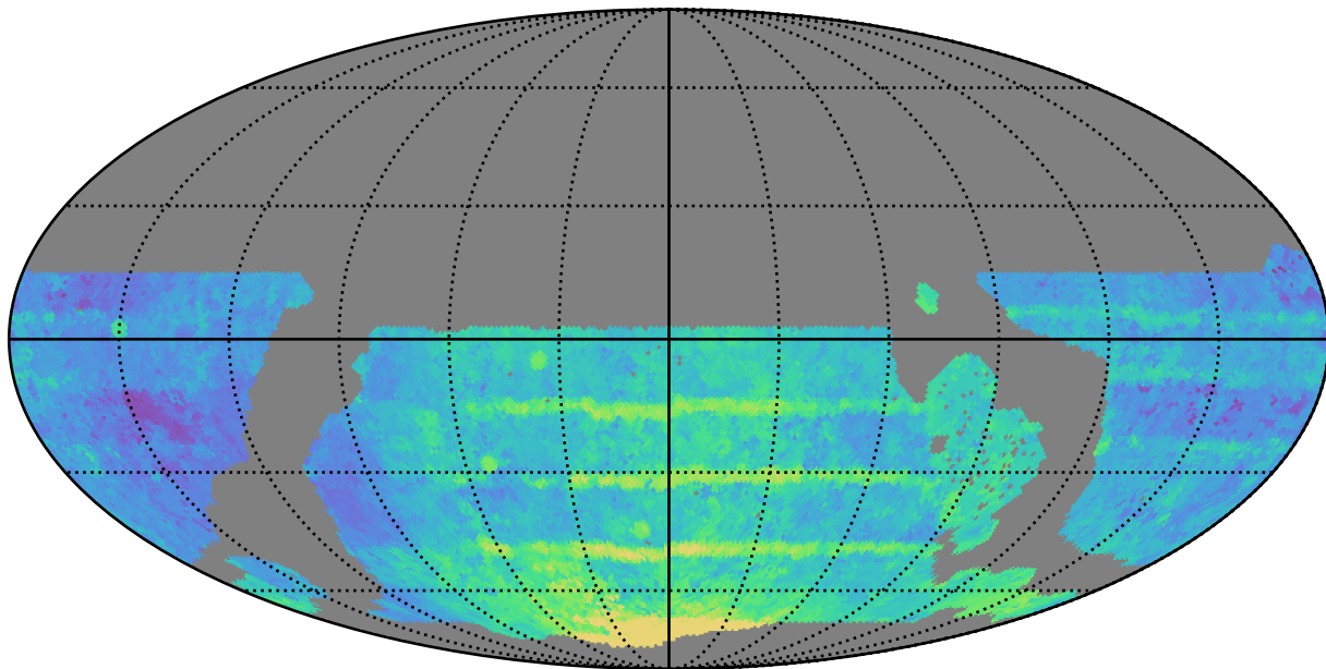
weather_cloudso2v3.4_10yrs WFD all bands: Median Season Length
