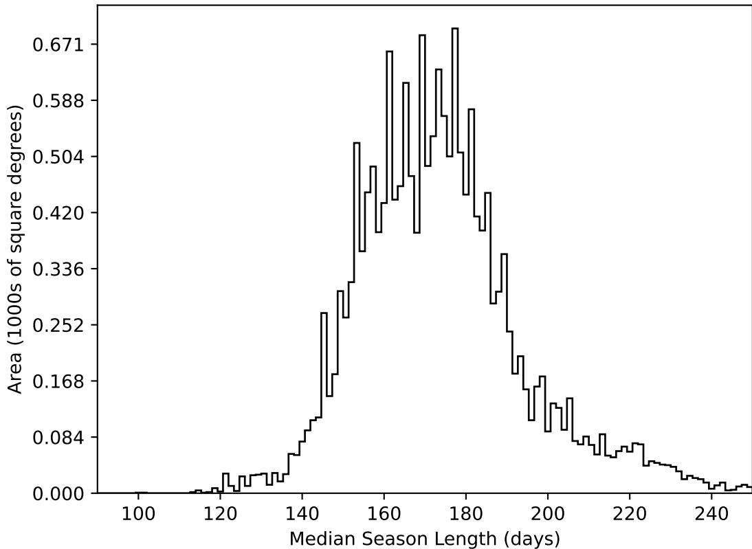
weather_cloudso2v3.4_10yrs WFD all bands: Median Season Length
