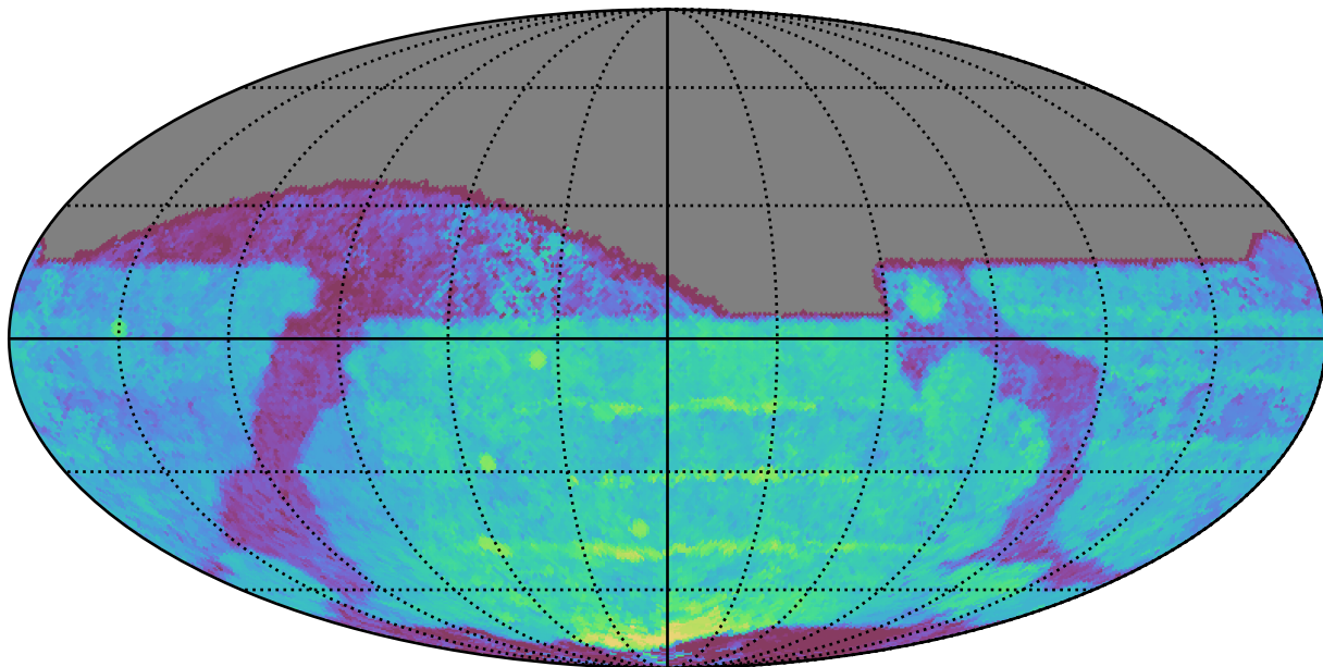
weather_cloudso2v3.4_10yrs All sky z band: Median Season Length
