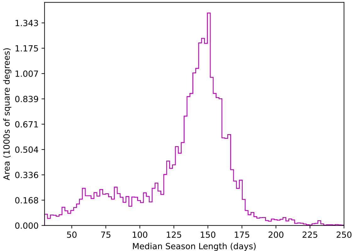
weather_cloudso2v3.4_10yrs All sky z band: Median Season Length
