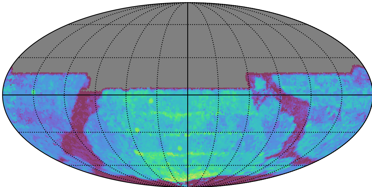
weather_cloudso2v3.4_10yrs All sky y band: Median Season Length
