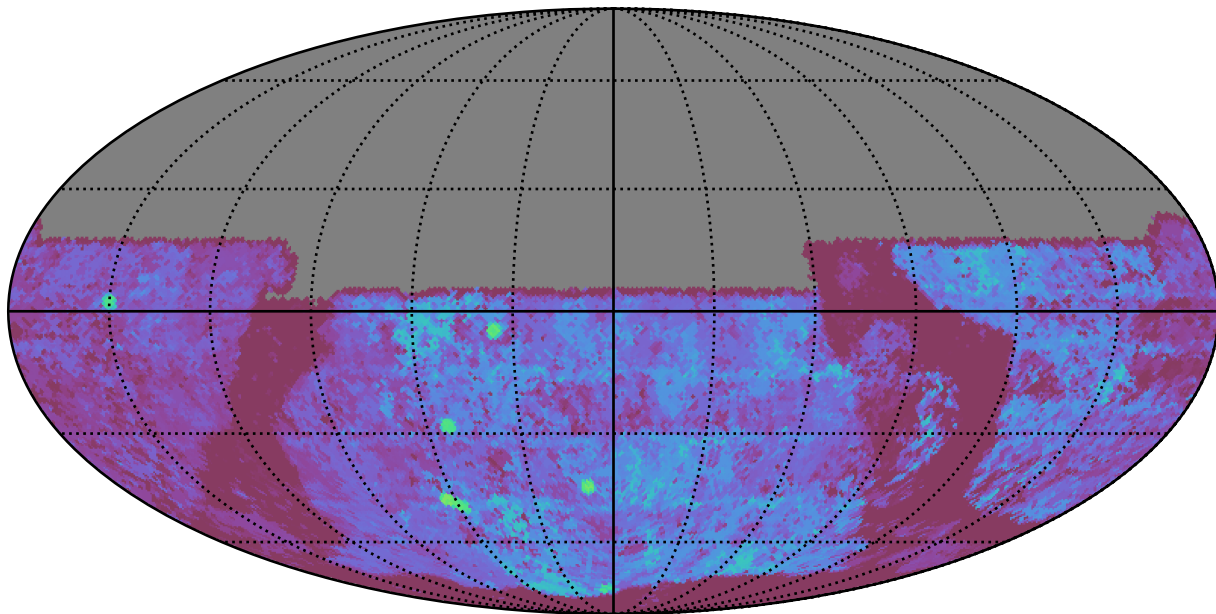
weather_cloudso2v3.4_10yrs All sky u band: Median Season Length
