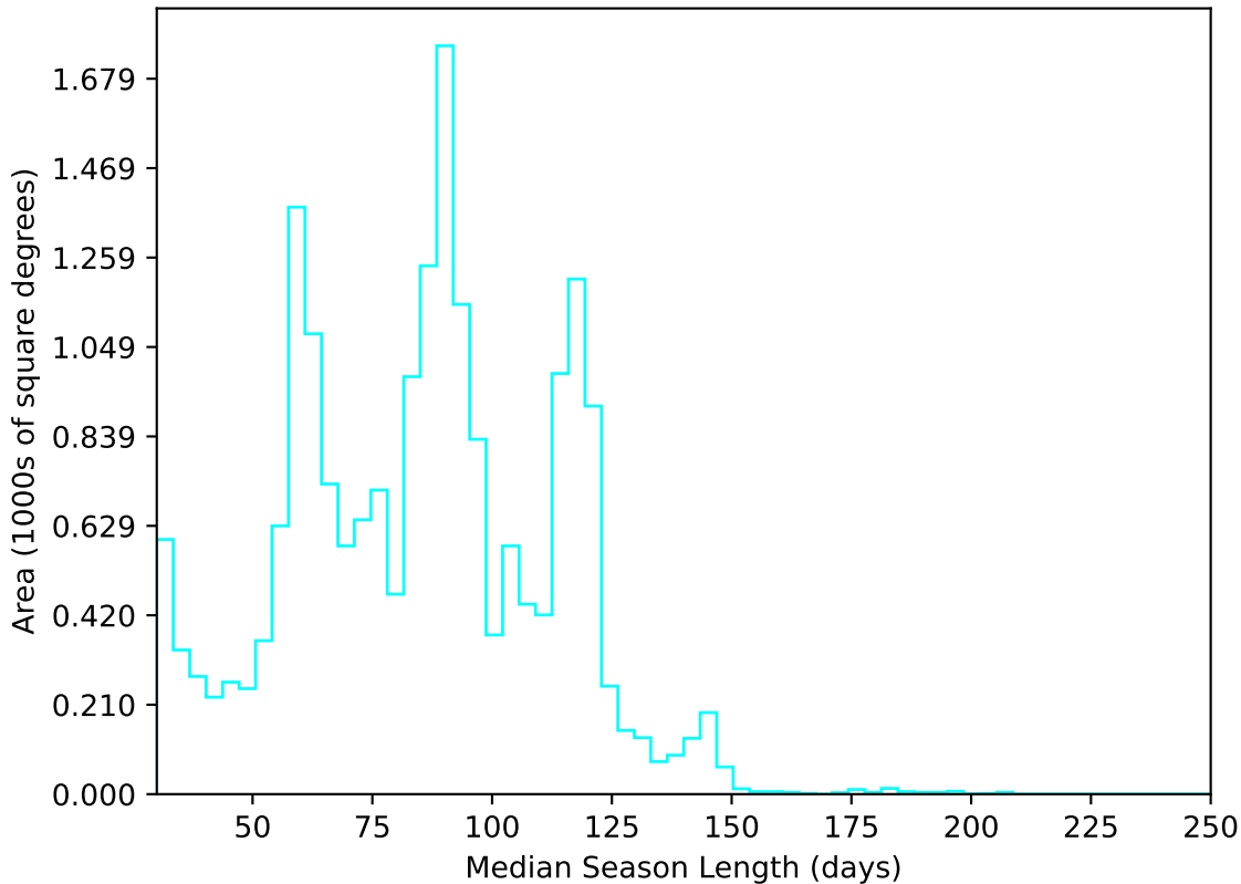
weather_cloudso2v3.4_10yrs All sky u band: Median Season Length
