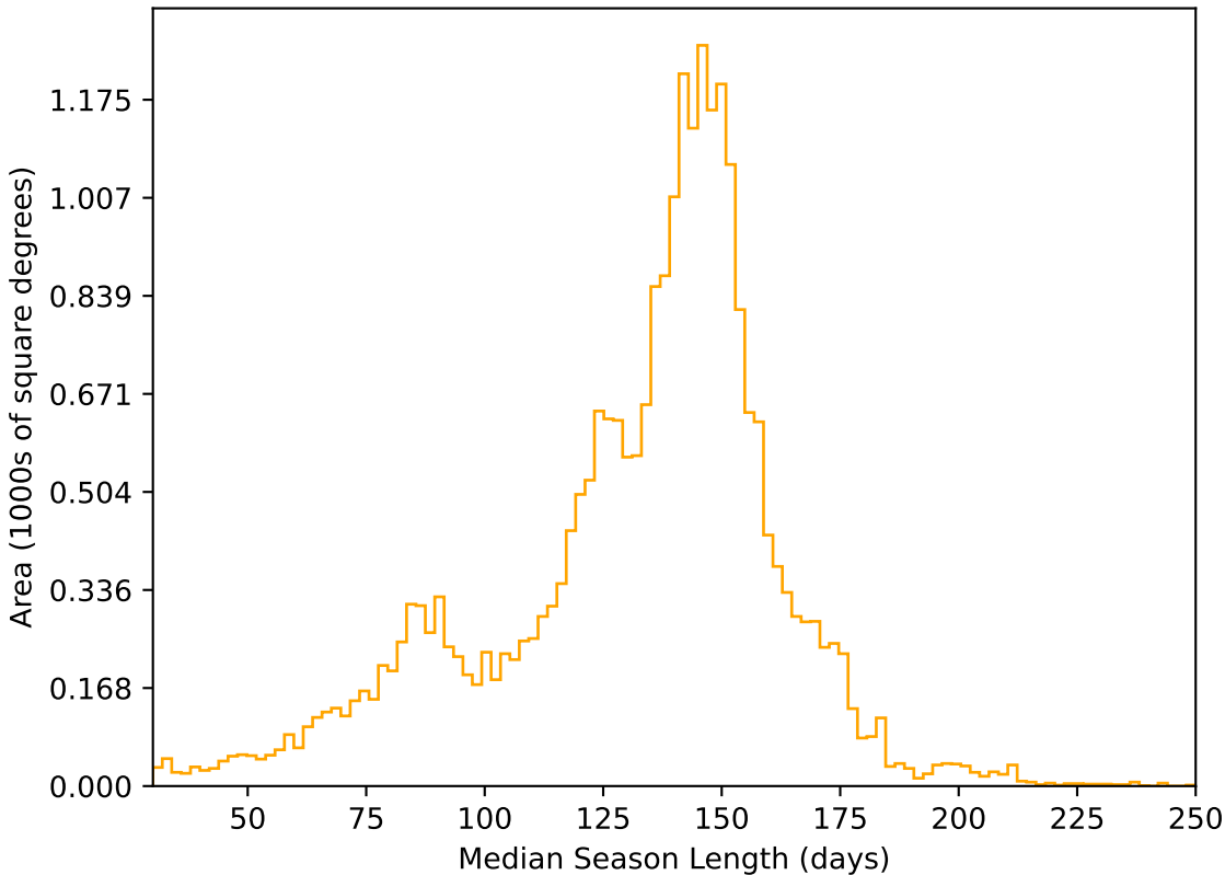
weather_cloudso2v3.4_10yrs All sky r band: Median Season Length
