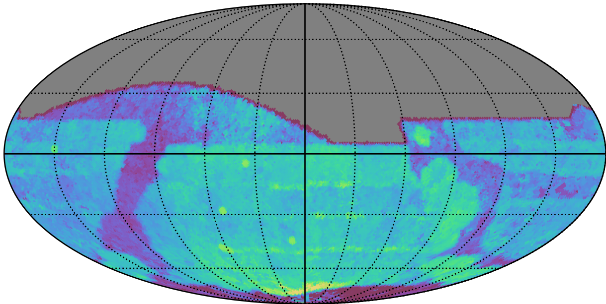
weather_cloudso2v3.4_10yrs All sky i band: Median Season Length
