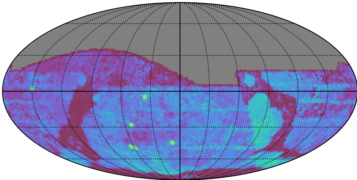
weather_cloudso2v3.4_10yrs All sky g band: Median Season Length
